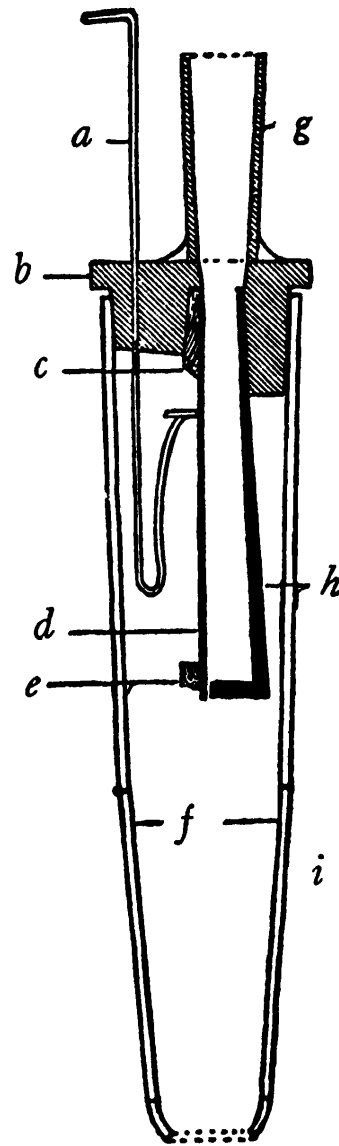
FIGURE 85. Reed pipe. a tuning spring, b block, c wedge, d vibrating tongue, e weight, f boot or socket, g shank, h shalet, i section of a reed.
